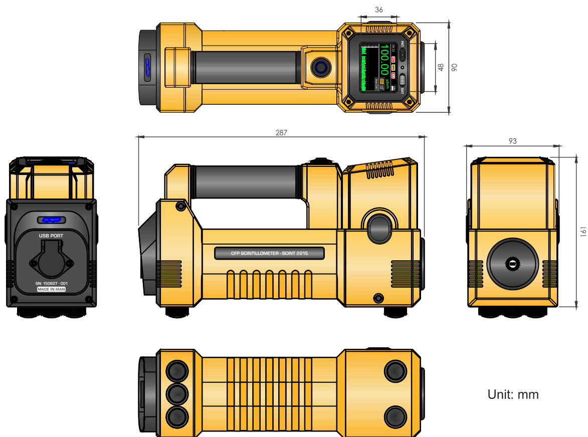
SCINT2215-Mechanical
